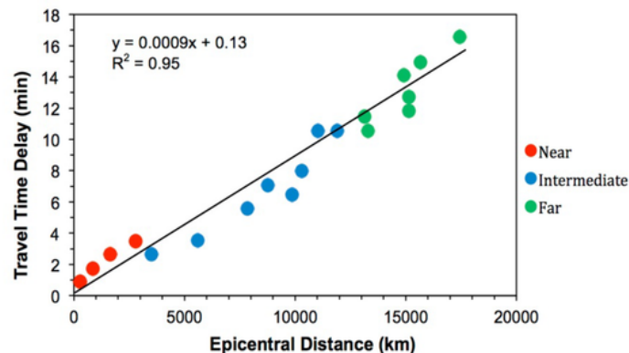
Figure 3. Travel time delay as a function of epicentral distance for the 2014 Chilean event.
